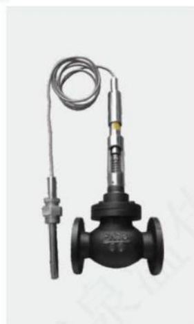
ZZWP 自力式温度调节阀 Self operated temperature control valve
